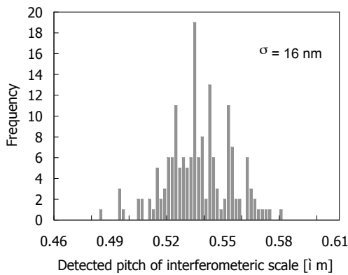
Fig. 1: Histogram of the detected pitches of the interferometric scale by the probe
